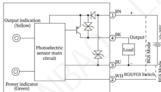
PNP
